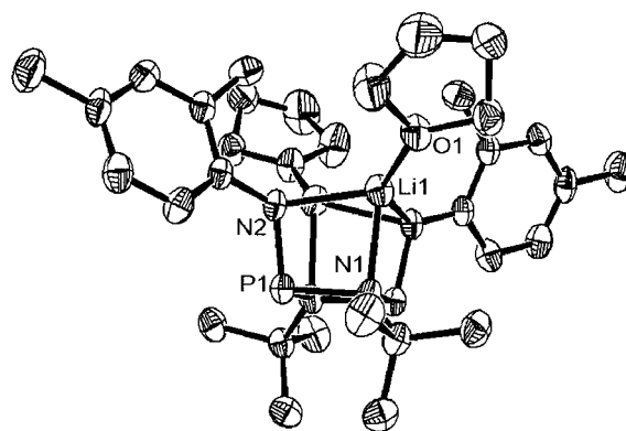
Figure 4. ORTEP diagram of cis -[(2,4-Me 2 \text{C}_6\text{H}_3\text{N} )(PN- t Bu)] 2 Li 2 (THF) 2 ( 9 ); one solvent molecule is omitted for clarity
