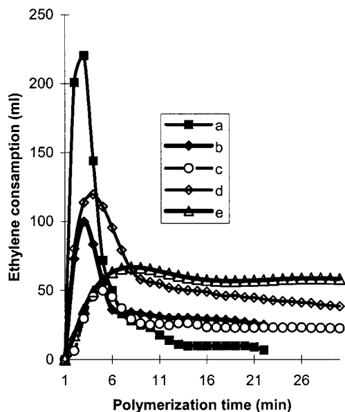
Figure 6. Ethylene consumption curves from polymerization experiments with (a) [(t\text{BuN})(t\text{BuNP})_2\text{TiCl}_2] ( 10 ), (b) [(\text{Ph}_2\text{CHN})(t\text{BuNP})_2\text{TiCl}_2] ( 12 ), (c) [(2,6\text{-Et}_2\text{PhN})(t\text{BuNP})_2\text{TiCl}_2] ( 13 ), (d) [(2,6\text{-}i\text{Pr}_2\text{PhN})(t\text{BuNP})_2\text{TiCl}_2] ( 14 ), and (e) [(2,5\text{-}t\text{Bu}_2\text{PhN})(t\text{BuNP})_2\text{TiCl}_2] ( 15 ) as catalyst precursors
