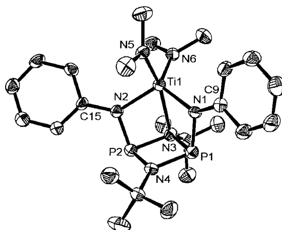
Figure 5. ORTEP diagram of cis –[(PhN)(PN- t Bu)] 2 Ti(NMe 2 ) 2 ( 11a )
