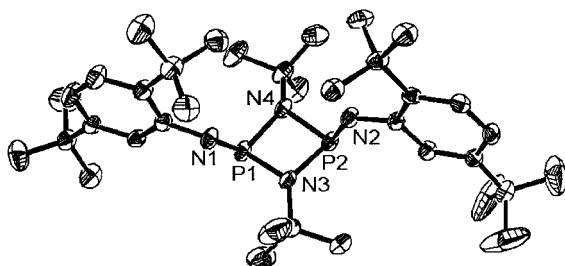
Figure 3. ORTEP diagram of cis -[(2,5-di- t Bu \text{C}_6\text{H}_3\text{NH} )(PN- t Bu)] 2 ( 5 )
