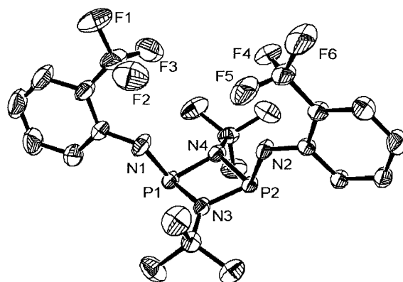
Figure 2. ORTEP diagram of cis -[(2- \text{CF}_3\text{C}_6\text{H}_4\text{NH})(\text{PN-}t\text{Bu})] 2 ( 4 )
