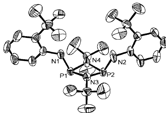
Figure 1. ORTEP diagram of cis -[(2- t BuC 6 H 4 NH)(PN- t Bu)] 2 ( 3 )
